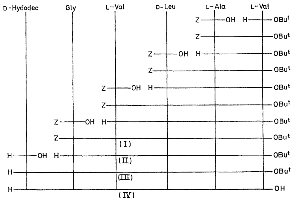
SCHEME Here and elsewhere abbreviations for amino-acid residues, etc. , are those recommended by I.U.P.A.C.-I.U.B. ( Biochem. J. , 1972, 126 , 773).
